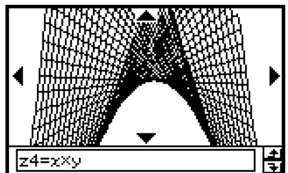
xgrid = 40, ygrid = 40
